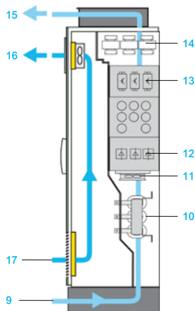
IP 54机柜
